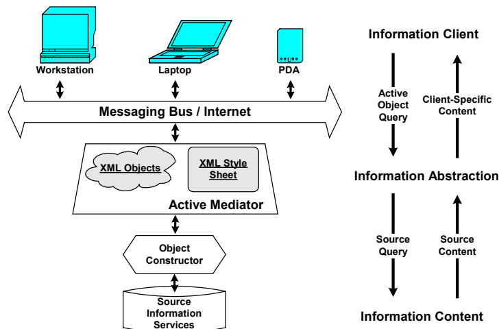
Figure 6: Active Mediation in Information Service Construction
