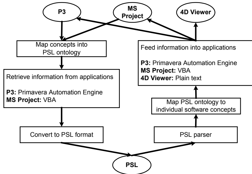
Figure 8: PSL Wrappers
