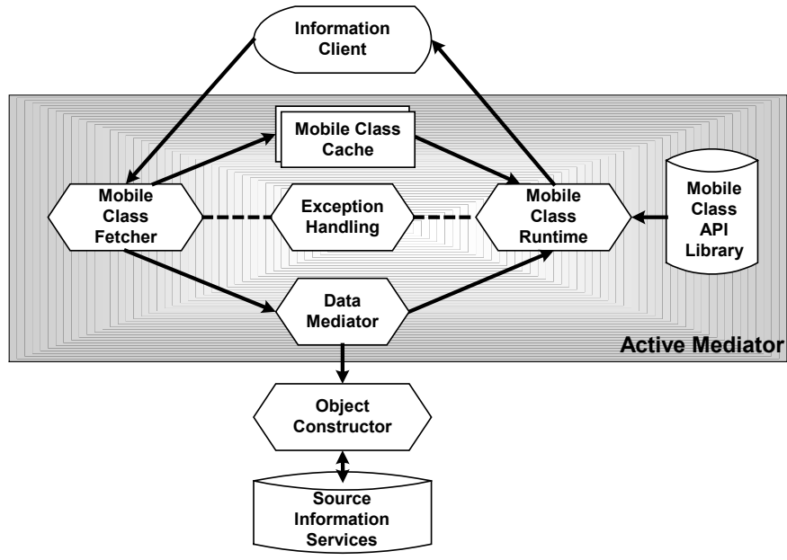
Figure 4: Active Mediation Architecture
