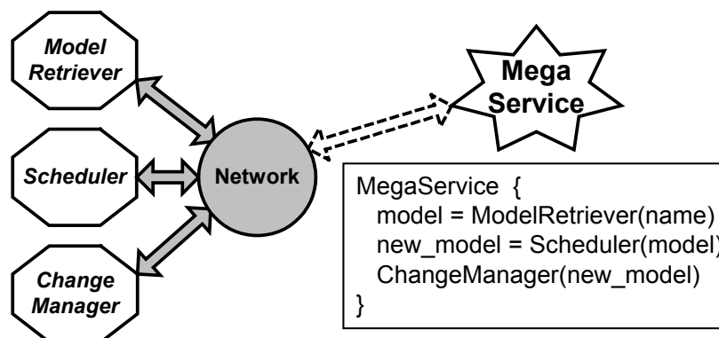
Figure 9: A Megaservice for Engineering Services
