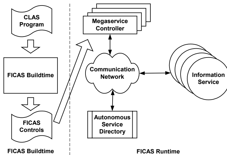
Figure 10: FICAS Architecture
