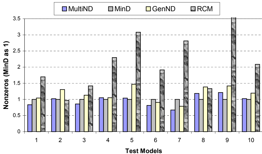
Figure 2.12: Quality Comparison of Different Matrix Ordering Schemes
