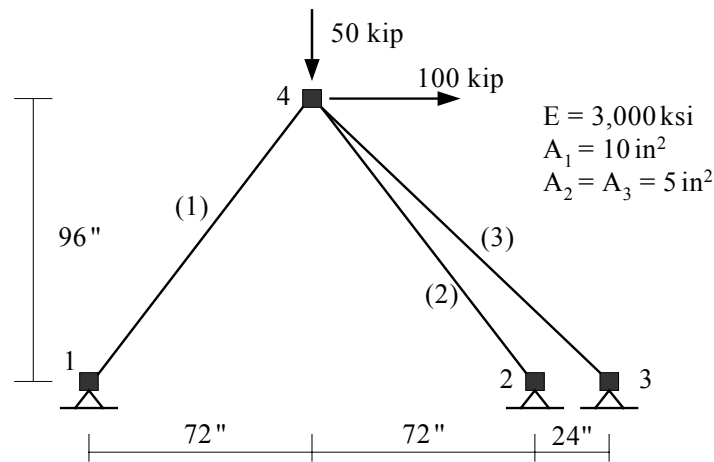
Figure 3.4: The Three-Truss Example (from [77])
