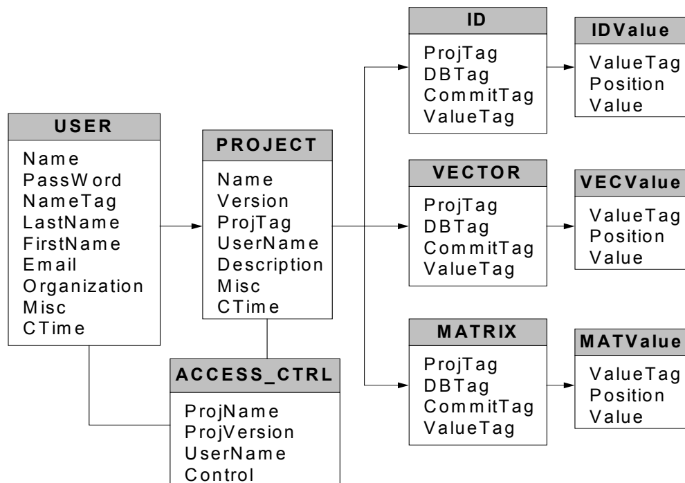
Figure 5.7: Database Schema Diagram for the Online Data Access System
