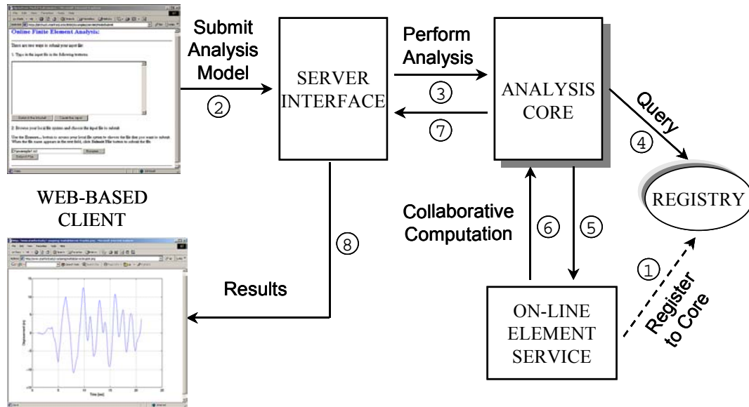
Figure 3.2: The Mechanics of the Collaborative Framework
