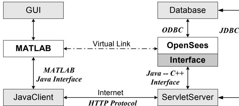
Figure 3.6: The Interaction Diagram for the MATLAB-Based Interface
