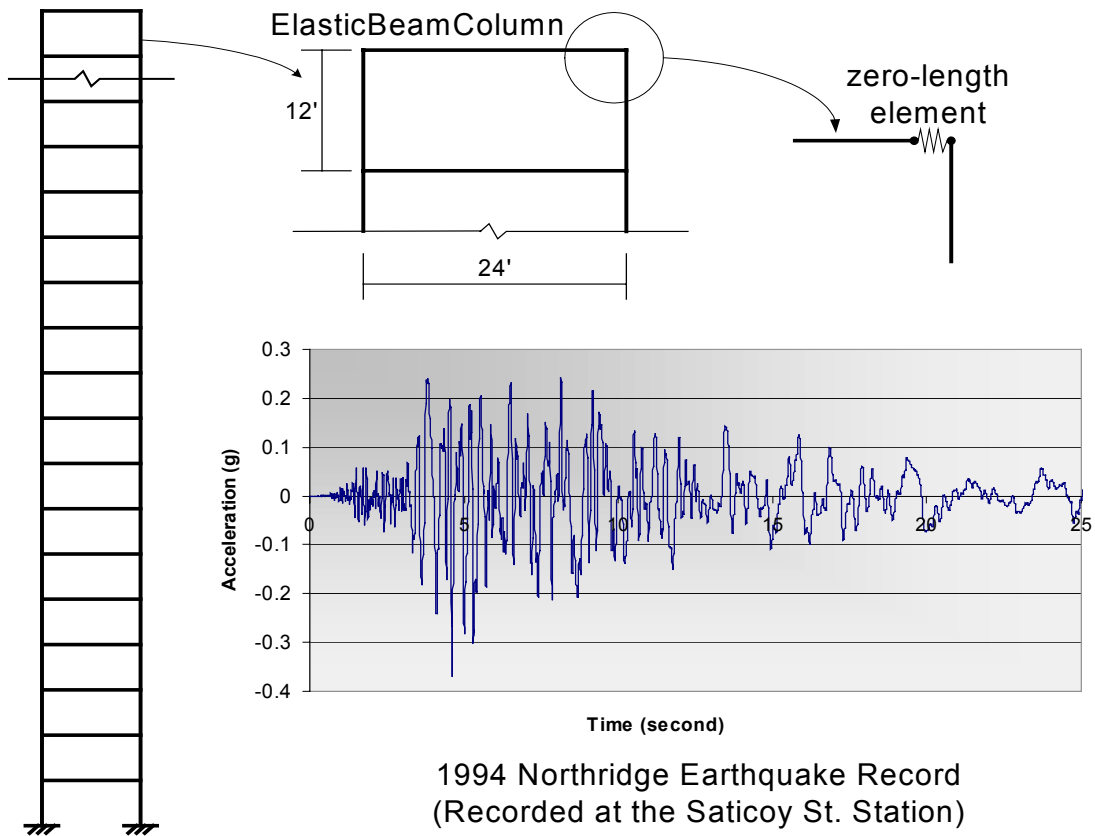
Figure 3.8: The Example Model and the Northridge Earthquake Record
