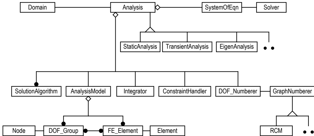
Figure 2.2: Class Diagram for OpenSees Analysis Framework (from [76])
