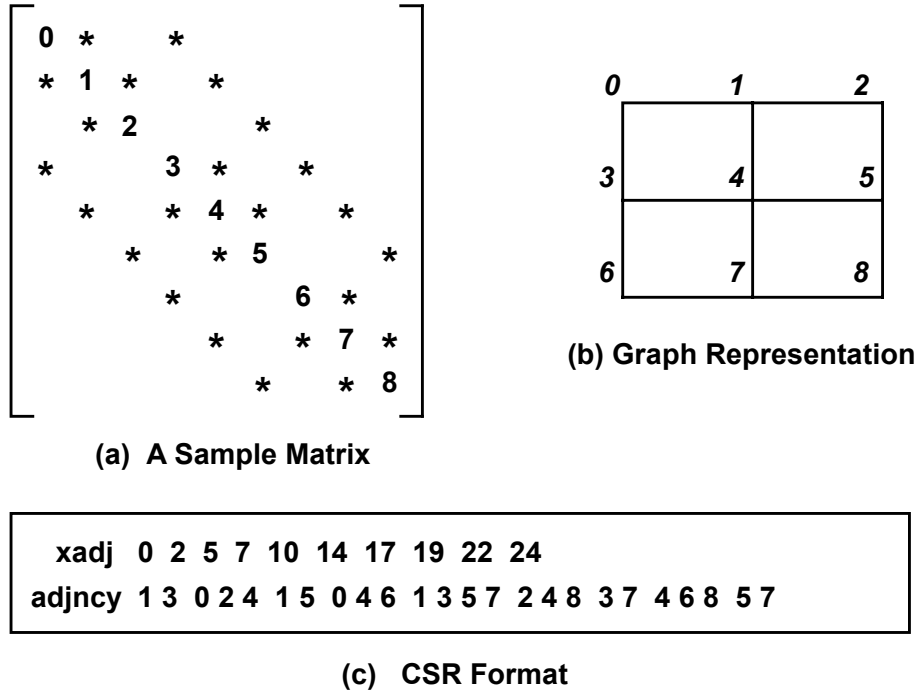
Figure 2.4: An Example of the CSR Storage for Matrix Structure
