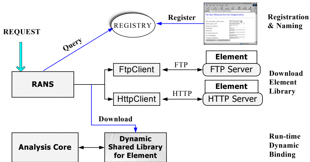
Figure 4.9: The Mechanics of Dynamic Shared Library Element Service
