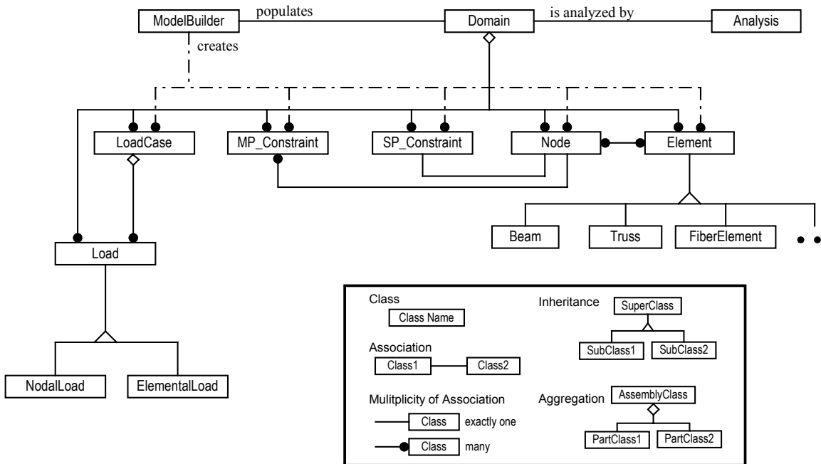
Figure 2.1: Class Abstraction in OpenSees (from [76])
