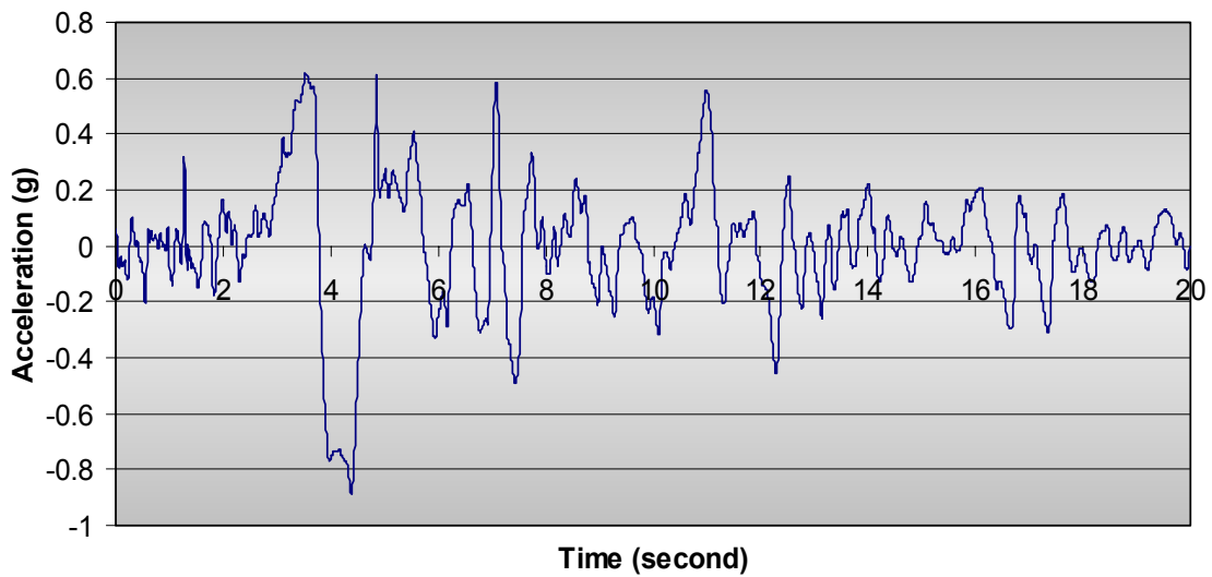
Figure 5.16: 1994 Northridge Earthquake Recorded at the Rinaldi Station
