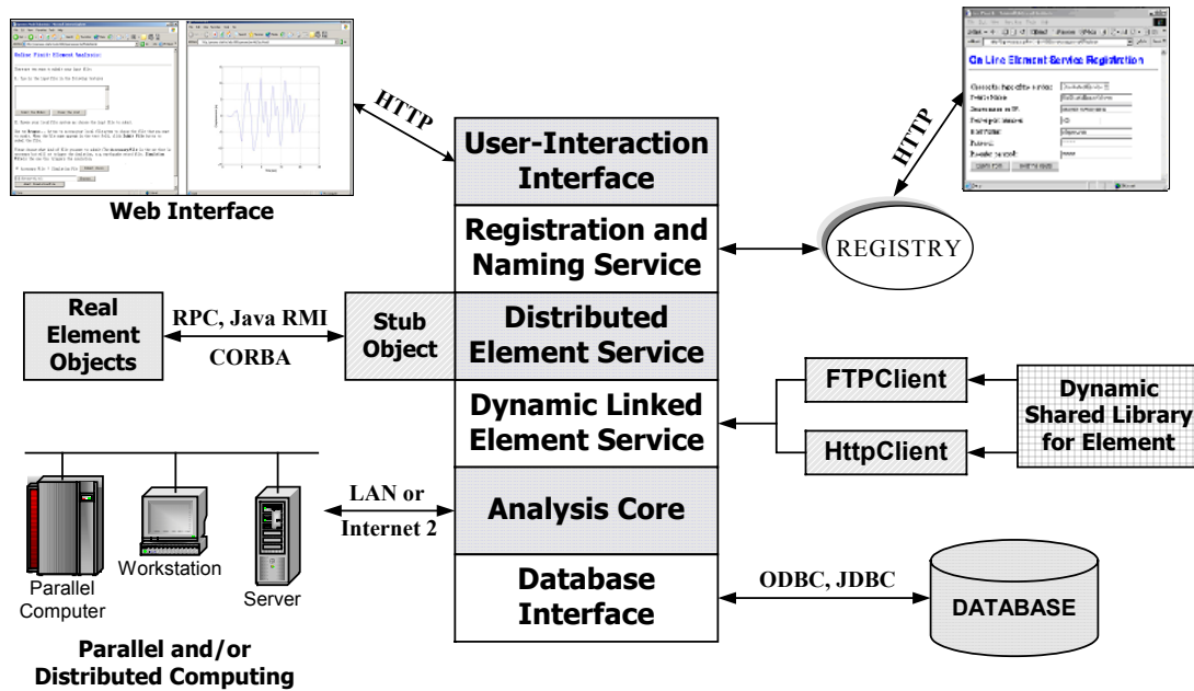
Figure 3.3: The Modules of the Collaborative System
