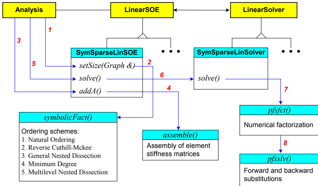
Figure 2.9: The Control Flow of Integrating the SymSparse Linear Solver
