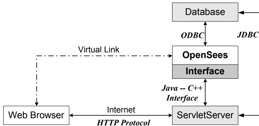
Figure 3.5: The Interaction Diagram for the Web-Based Interface
