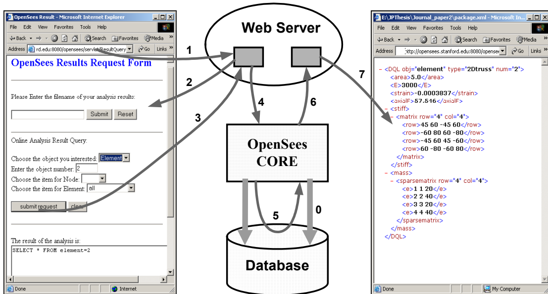
Figure 5.11: Interaction Diagram of Online Data Access System
