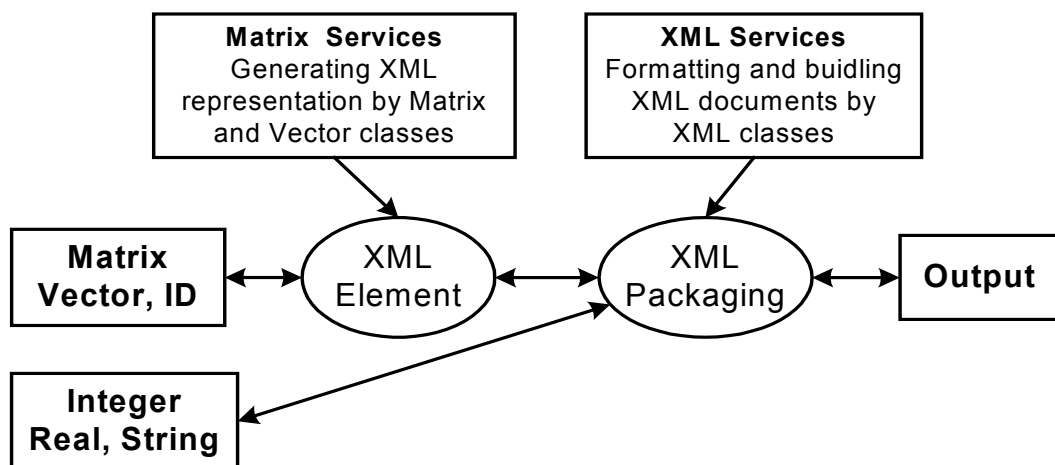
Figure 5.8: The Relation of XML Services
