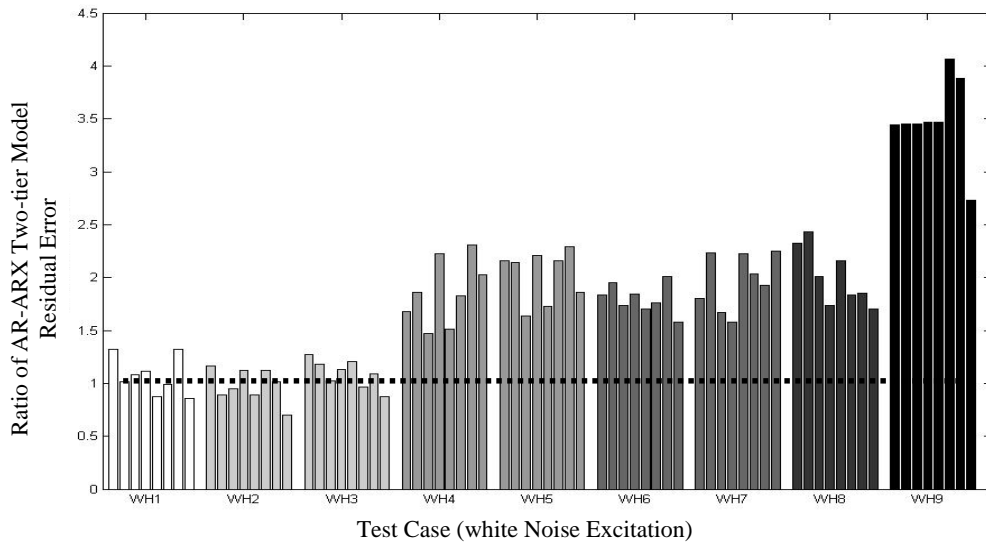
Figure 7a: Ratio of AR-ARX two-tier model residual error from test of pure RC frame.
