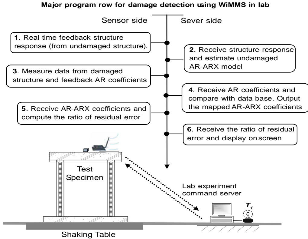
Figure 6: Implementation of the AR-ARX damage detection strategy in a wireless monitoring system to conduct the continuous damage detection of large structural testing in the laboratory.
