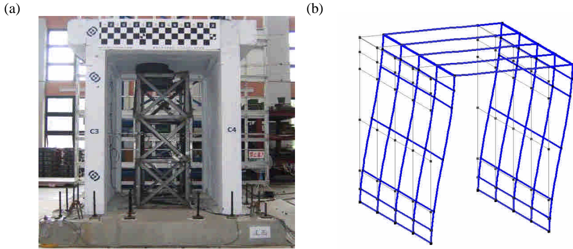
Figure 1: (a) Photo of the specimen B1F. (b) The first dominant mode of the frame structure.
