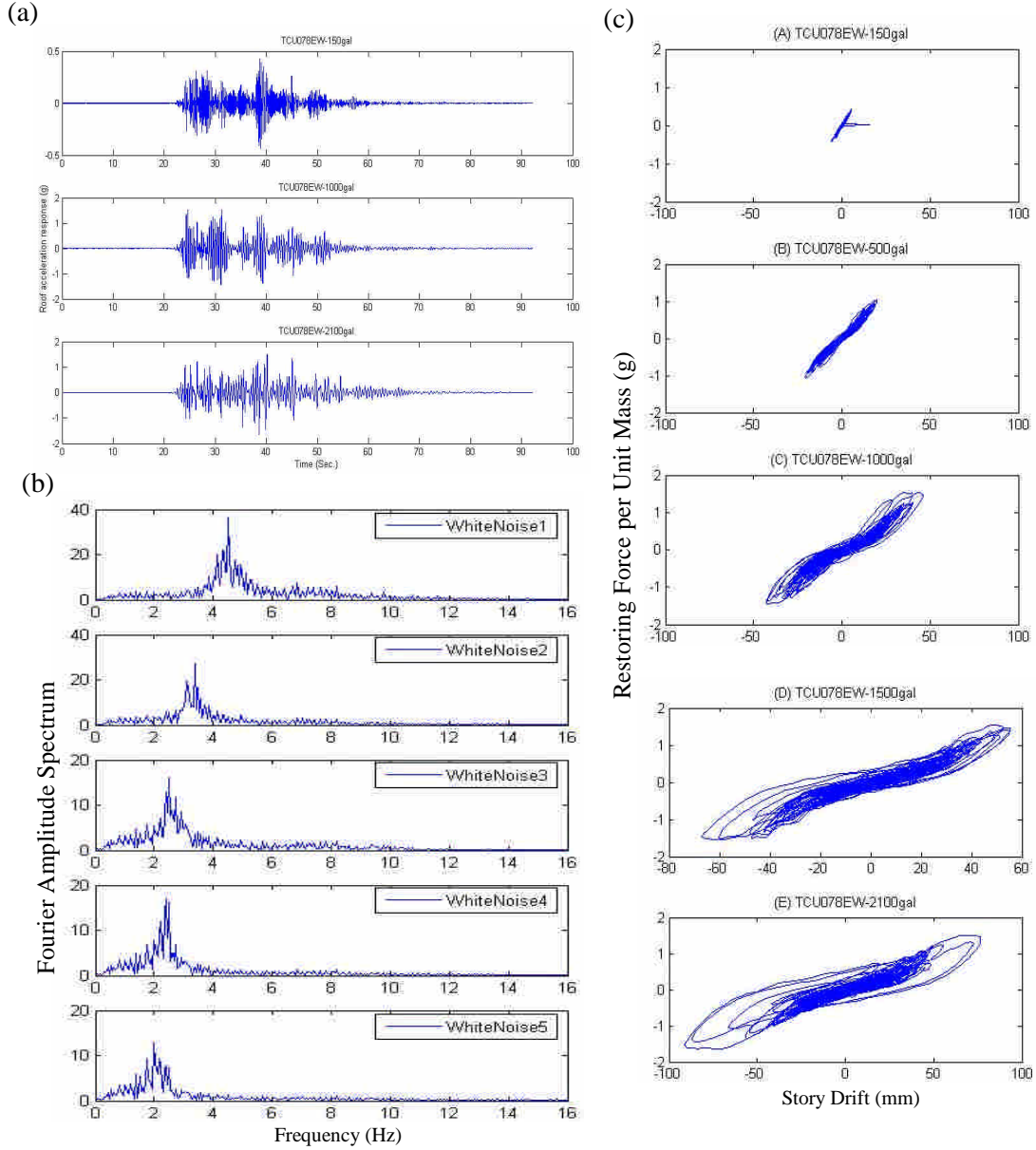
Figure 5b: Plot of floor acceleration responses, Fourier amplitude spectrum, and restoring force diagram from test case B (A1F); (a) Acceleration response for input PGA=150gal, 1000gal, and 2100 gal, (b) Fourier amplitude spectrum of ambient signal from different stage of test, (c) Restoring diagram of the test structure from different test stage.
