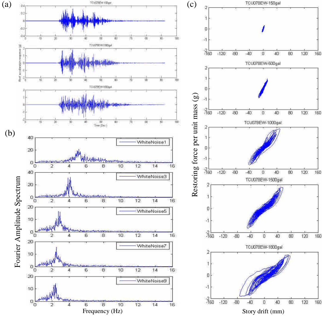
Figure 5a: Plot of floor acceleration responses, Fourier amplitude spectrum, and restoring force diagram from test case A (PF); (a) Acceleration response for input PGA=150gal, 1000gal, and 1800 gal, (b) Fourier amplitude spectrum of ambient signal from different stage of test, (c) Restoring diagram of the test structure from different test stage.
