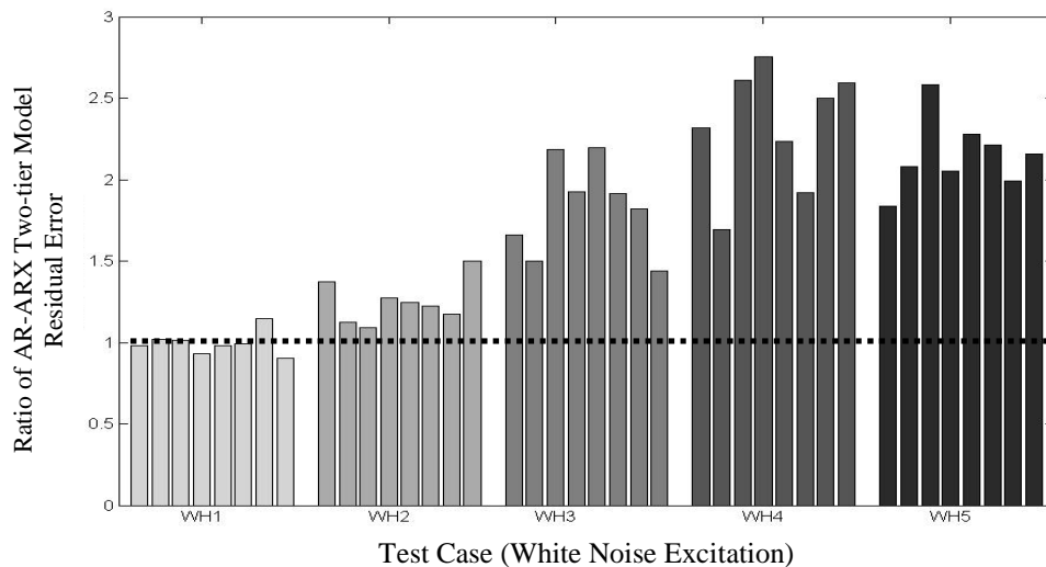
Figure 7b: Ratio of AR-ARX two-tier model residual error from test of RC frame in filled with 1/2B post-laid brick walls.
