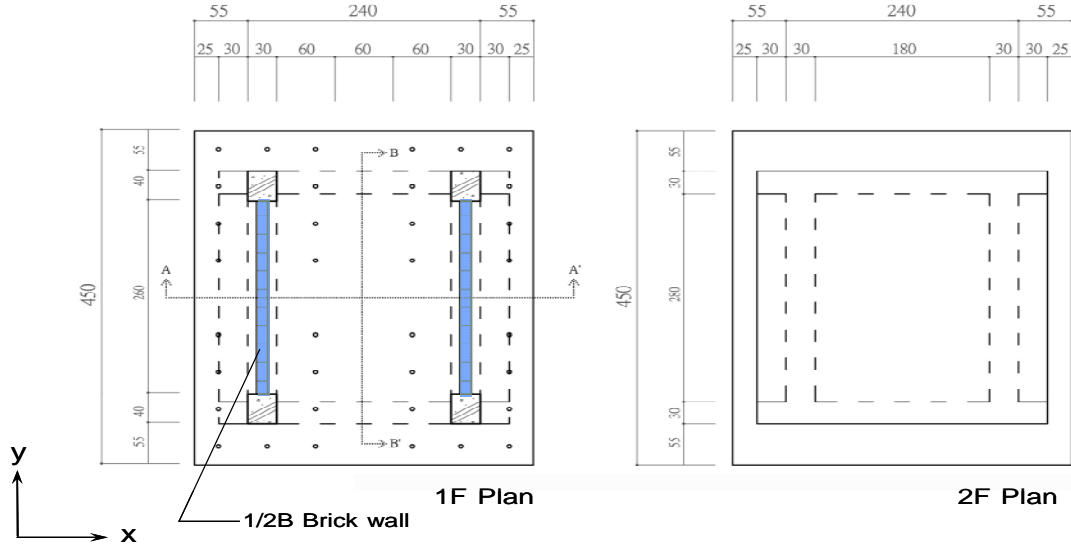
Figure 2a: Top view of the test specimen (A1F).
