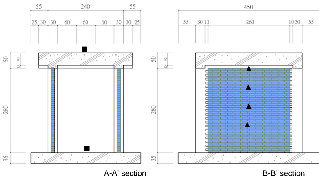
Figure 2b: Side view of the test specimen. Locations of accelerometers (■) and LVDT (▲) are also shown.
