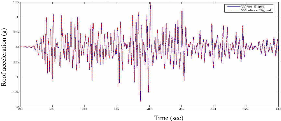
Figure 3: Comparison on roof response of the test specimen to Chi-Chi TCU078(1800 gal) strong motion from both conventional accelerometer and wireless sensing unit
