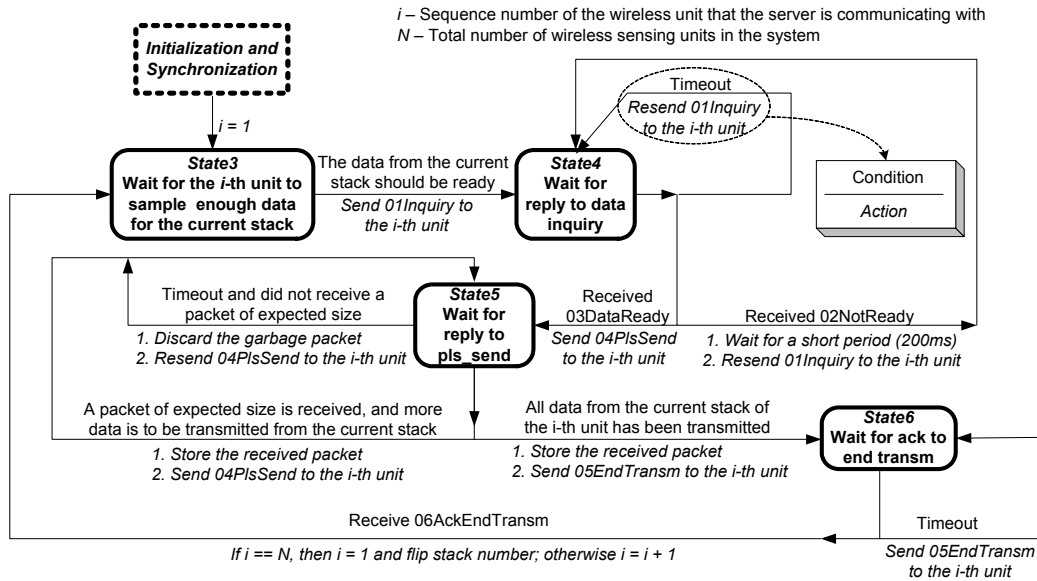
Fig. 4. Communication state diagram of the server.
