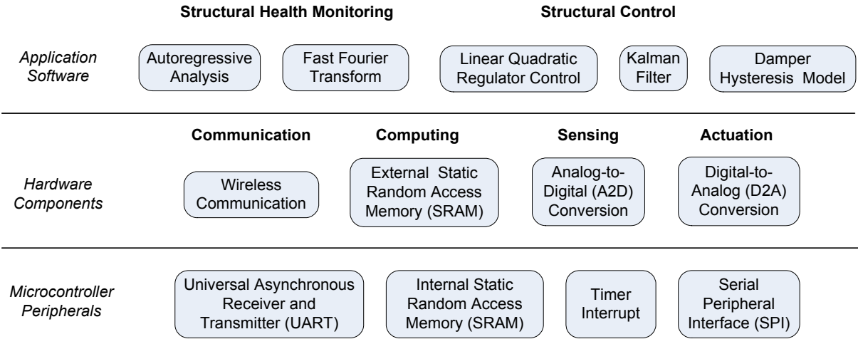
Fig. 2. Software layers of the ATmega128 microcontroller in the wireless sensing and actuation unit.
