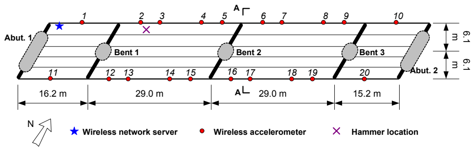
(a) Plan view of the bridge illustrating locations of wireless accelerometers.
