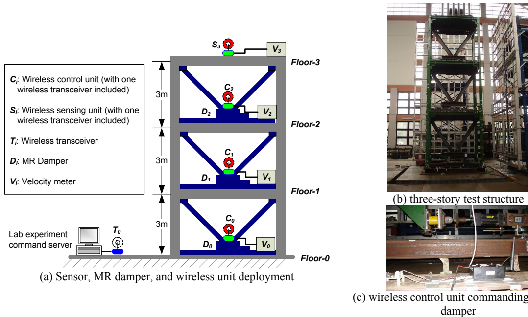
Fig. 10. Laboratory setup of the wireless structural control system.
